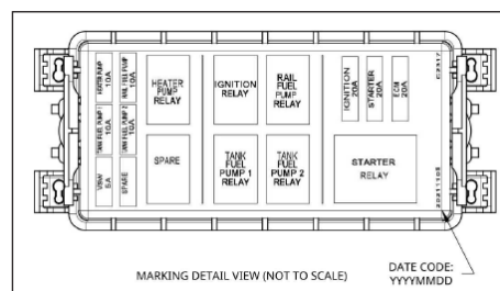
M5/M6 Fuse Box Diagram
