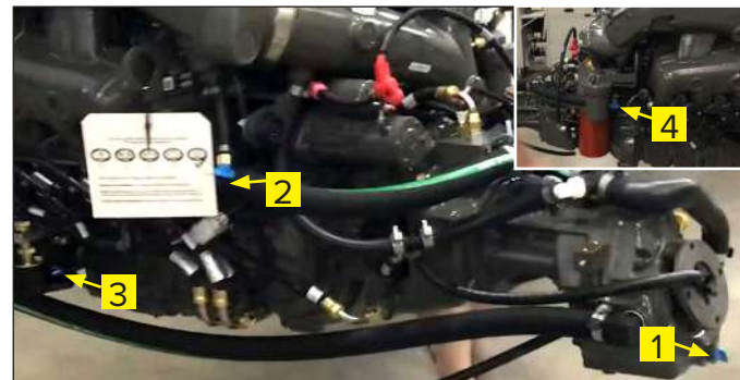
The engine drain plugs are located: 1. The V-Drive. 2. The bank 1 manifold. 3. Under the heat exchanger. 4. The bank 2 manifold.
