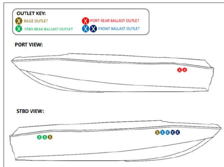
Figure 2: Outlet Diagram
