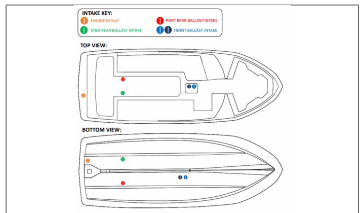
Figure 1: Axis Intake Diagram
