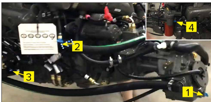
Drain Plug Locations – M5/M6
