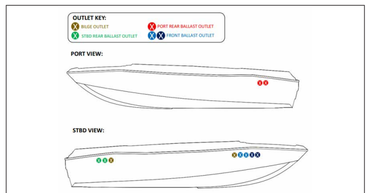
Figure 2: Axis Outlet Diagram
