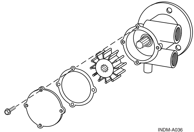
Figure 6.8 – Raw Water Pump Impeller
