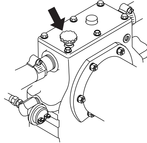
Figure 6.13 – Walters V-Drive Dipstick Location
