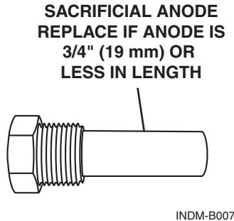
Figure 6.7 – Sacrificial Anode
